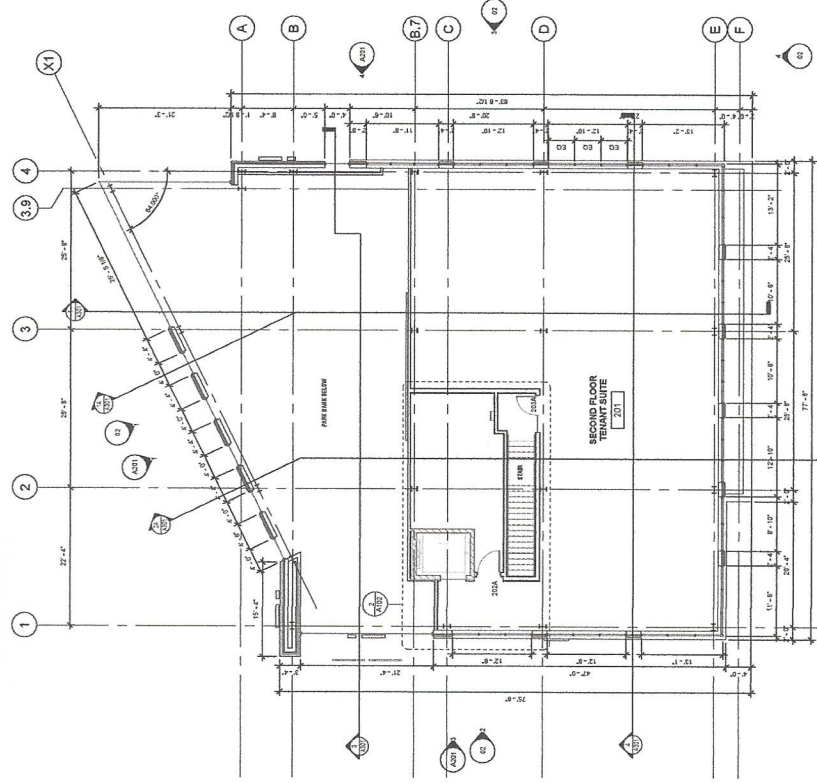
1 SECOND FLOOR PLAN 1/8" = 1'-0"
