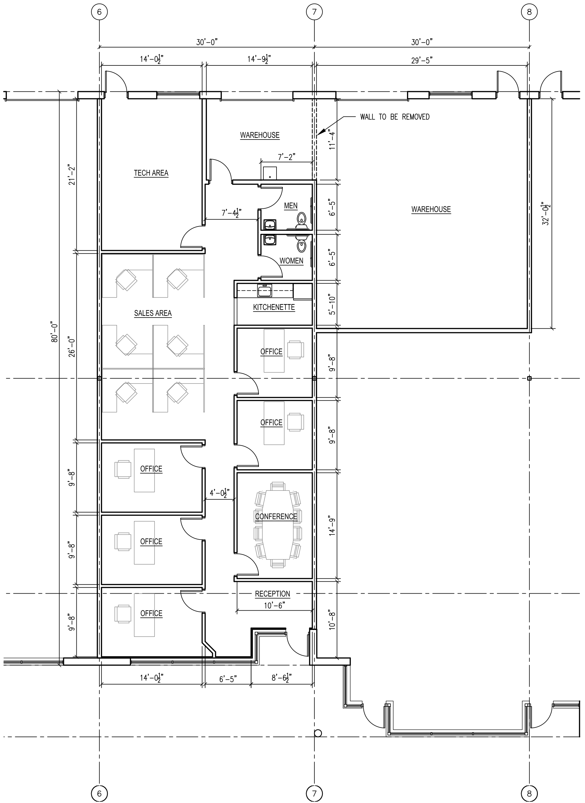
1 FLOOR PLAN 1/8" = 1'-0"
