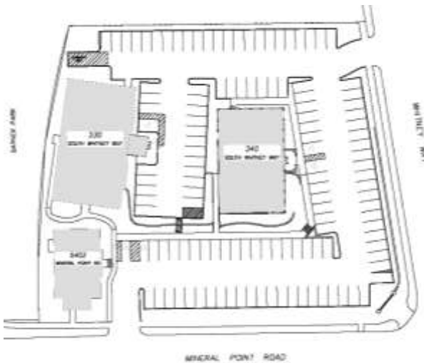
Whitney Point Site Plan
