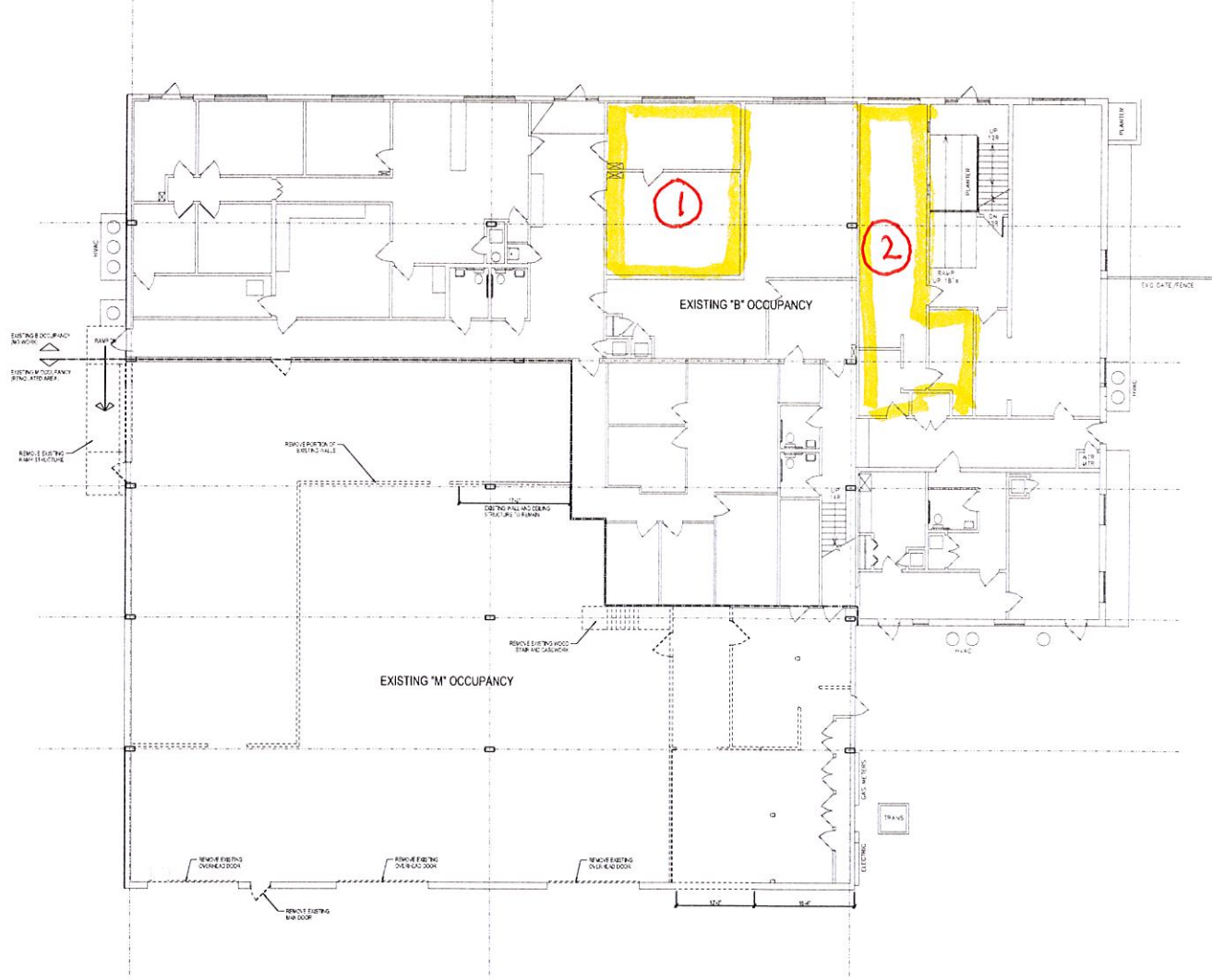
DEMOLITION FLOOR PLAN SCALE: 1/8"=1'-0"
