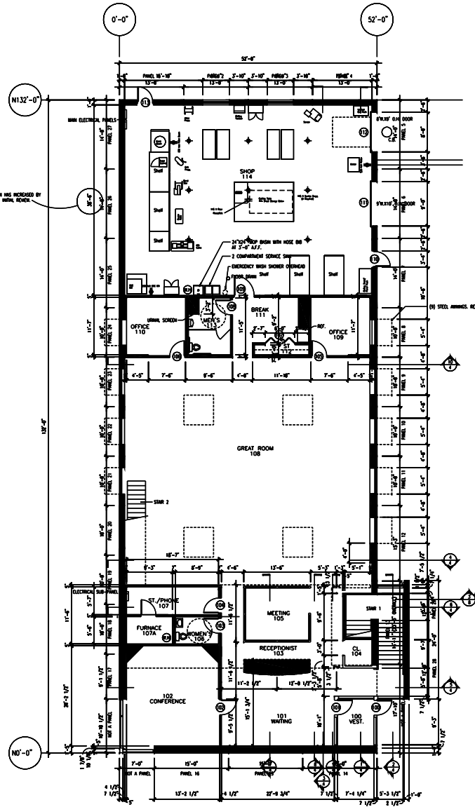
1C FIRST FLOOR PLAN SCALE: 1/8"=1'-0" 6300 S.F. FIRST FLOOR
