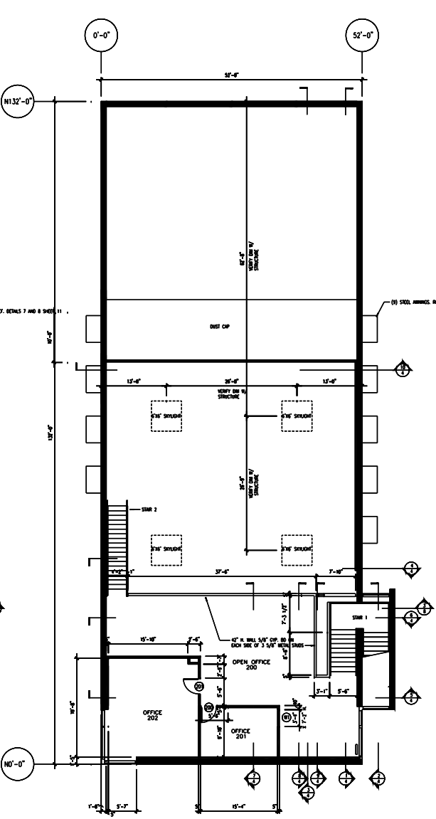
2C SECOND FLOOR PLAN SCALE: 1/8"=1'-0" 1473 S.F. SECOND FLOOR
