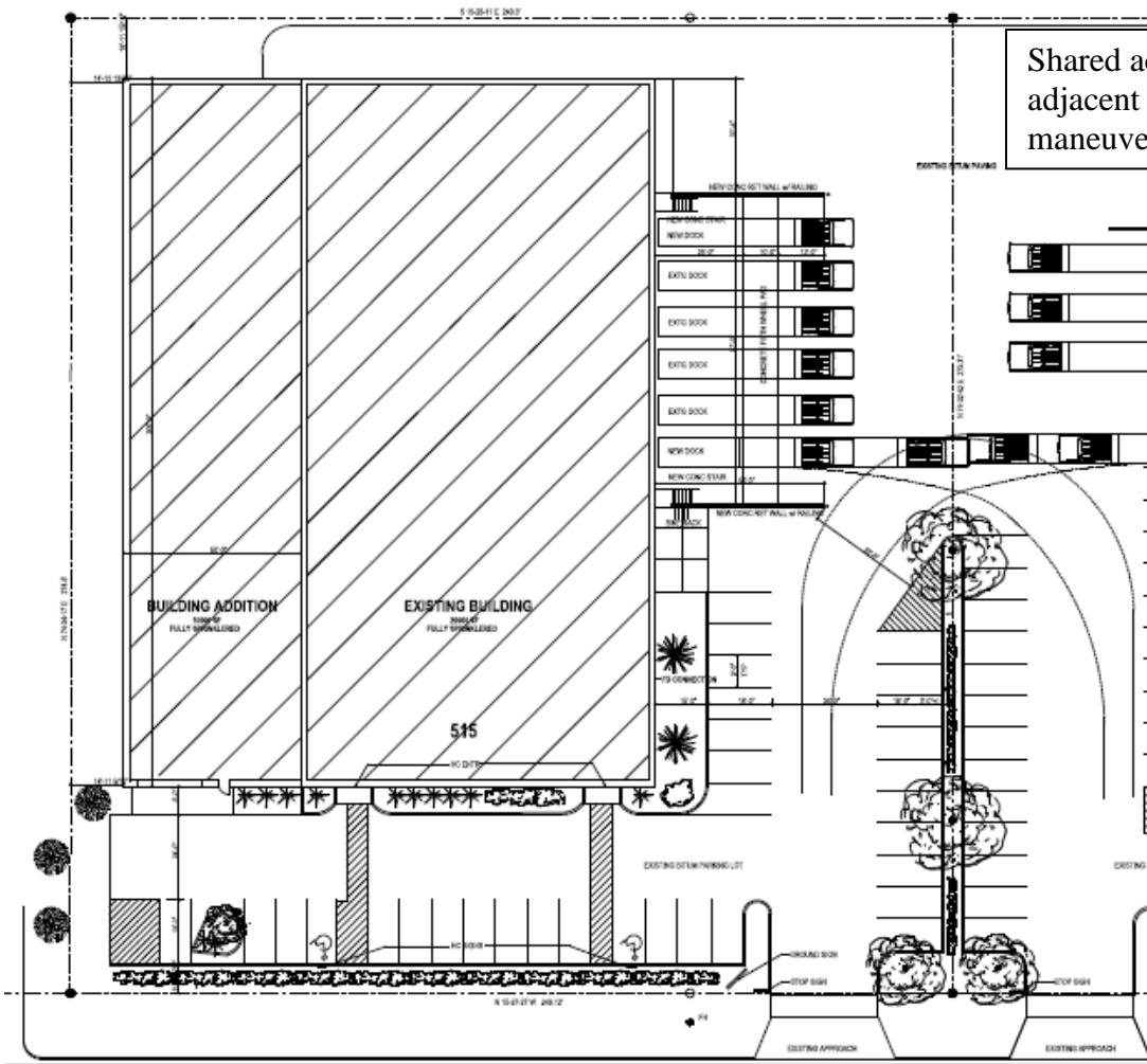
Site plan (showing potential 10,000 SF building addition)
