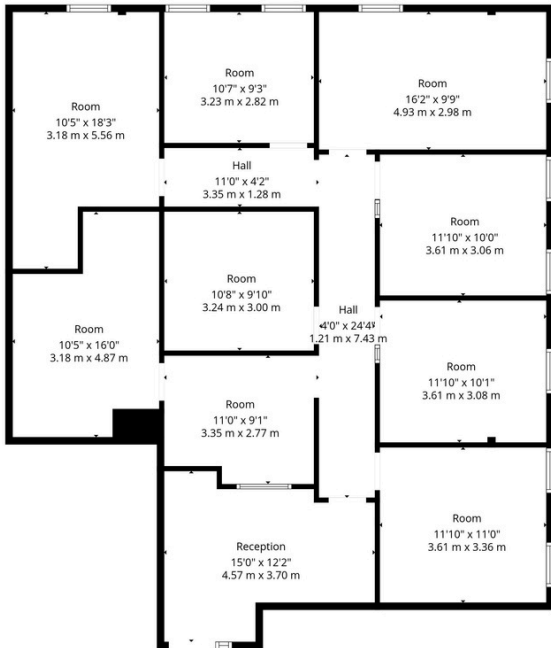
Total: 1482 sq. Ft. 138 m 2 1st Floor: 1482 sq. Ft. 138 m 2 Excluded Areas: Walls: 84 sq. Ft. 7 m 2 Measurements Deemed Highly Reliable But Not Guaranteed.
