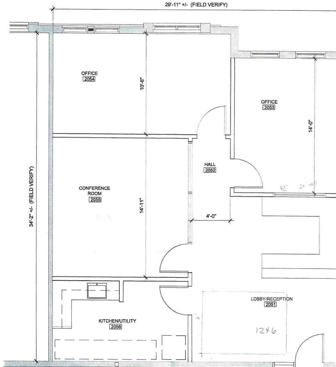
SUITE #205 FLOOR PLAN 1/4" = 1'-0" N
