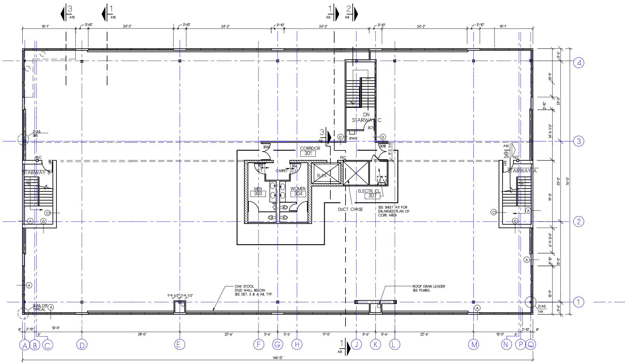
① THIRD FLOOR PLAN SCALE 1/8" = 1'-0"
