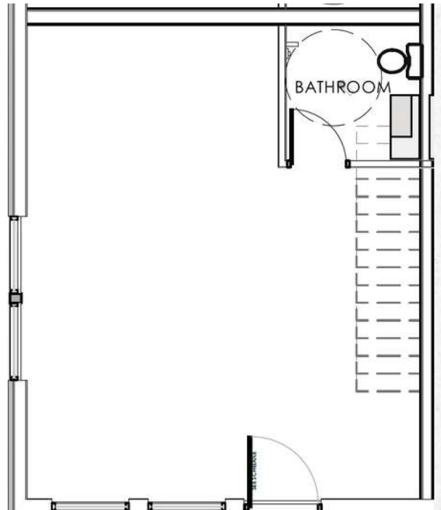
LOWER LEVEL/WORKSPACE
