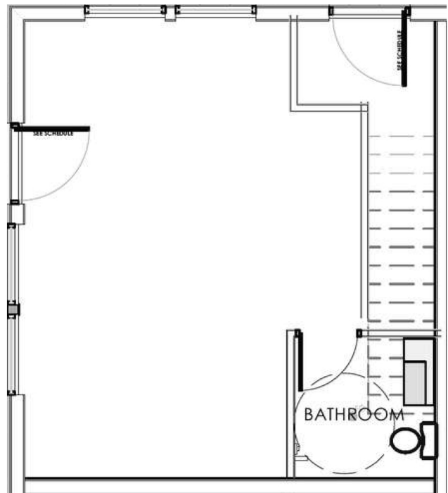
LOWER LEVEL/WORKSPACE
