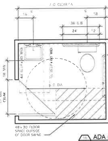
ADA COMPLIANT BATHROOM PLAN 2018/RECURS DESIGN & CONSTRUCTION INC. DRAWINGS DATE: 6/17/18
