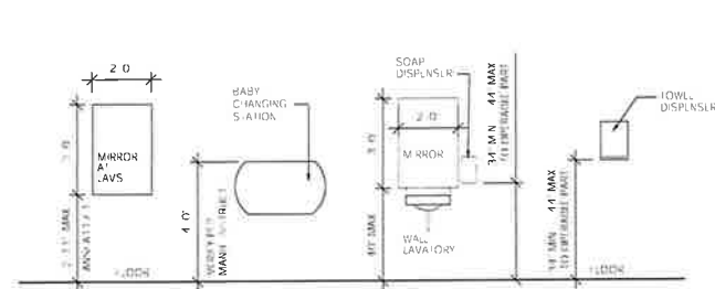
ADA COMPLIANT MOUNTING HEIGHTS 2018/RECURS DESIGN & CONSTRUCTION INC. DRAWINGS DATE: 6/17/18
