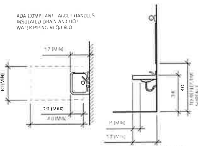
ADA COMPLIANT LAVATORY ELEVATIONS 2018/RECURS DESIGN & CONSTRUCTION INC. DRAWINGS DATE: 6/17/18
