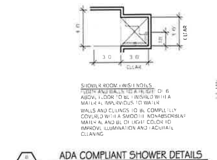
ADA COMPLIANT SHOWER DETAILS 2018/RECURS DESIGN & CONSTRUCTION INC. DRAWINGS DATE: 6/17/18
