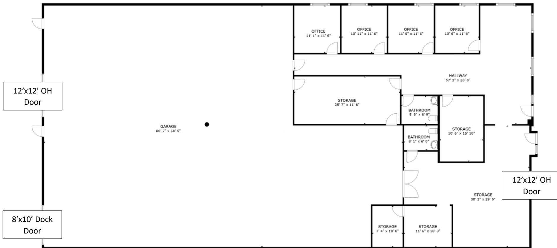
FLOOR PLAN
