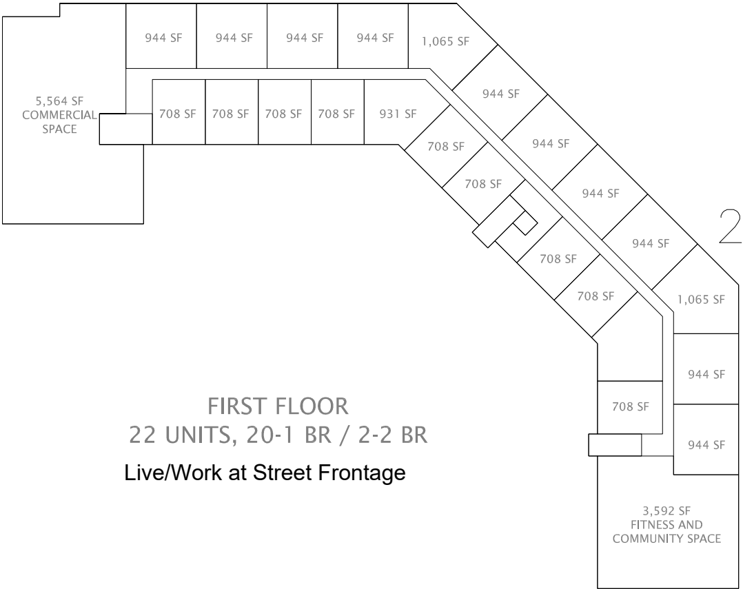
2525 BUILDING A 119 UNITS, 95-1 BR / 24-2 BR 159,670 GSF
