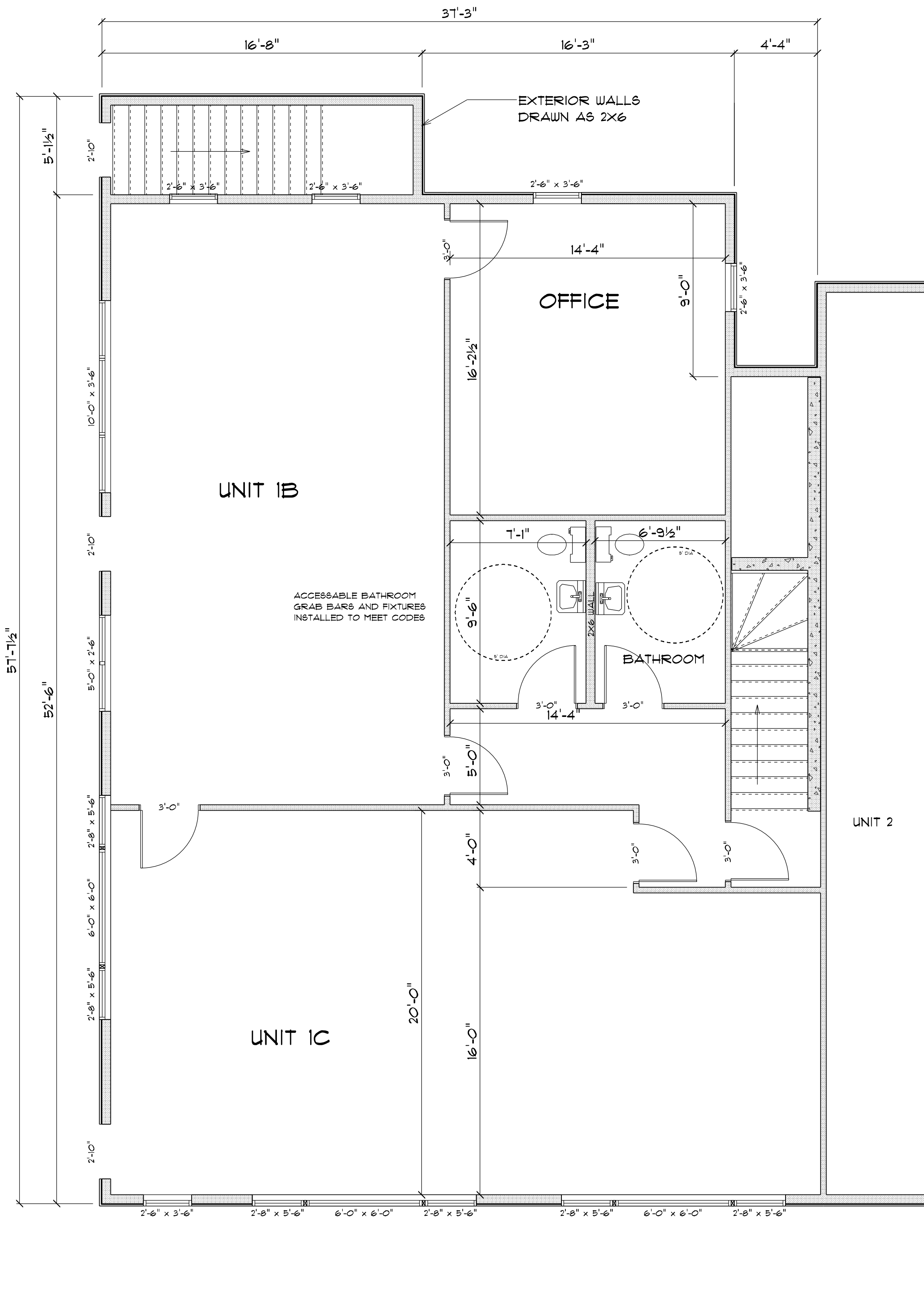
UNIT 1 BUILDOUT PLAN SCALE: 1/4" = 1'-0"
