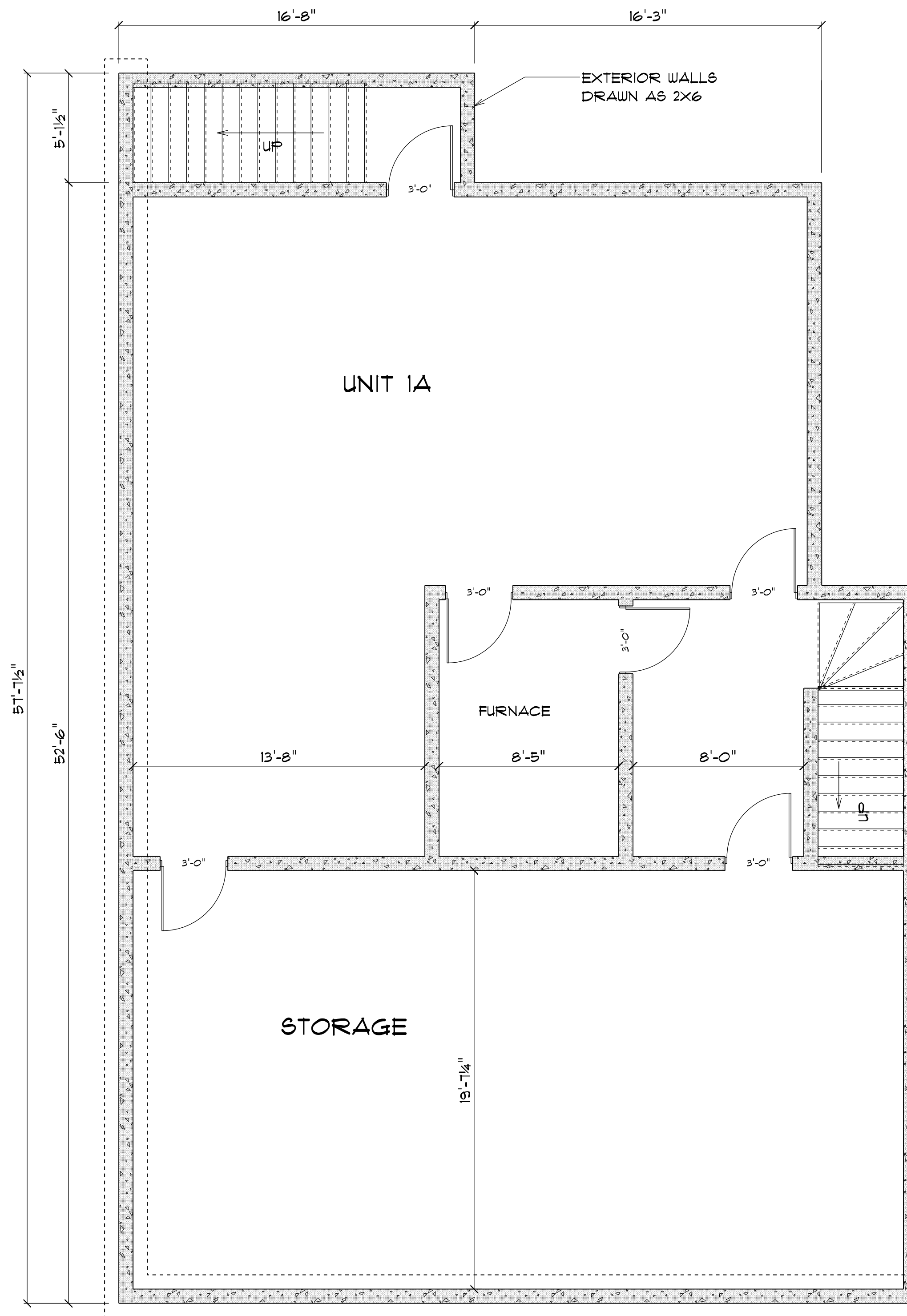
UNIT 1 BASEMENT SCALE: 1/4" = 1'-0"
