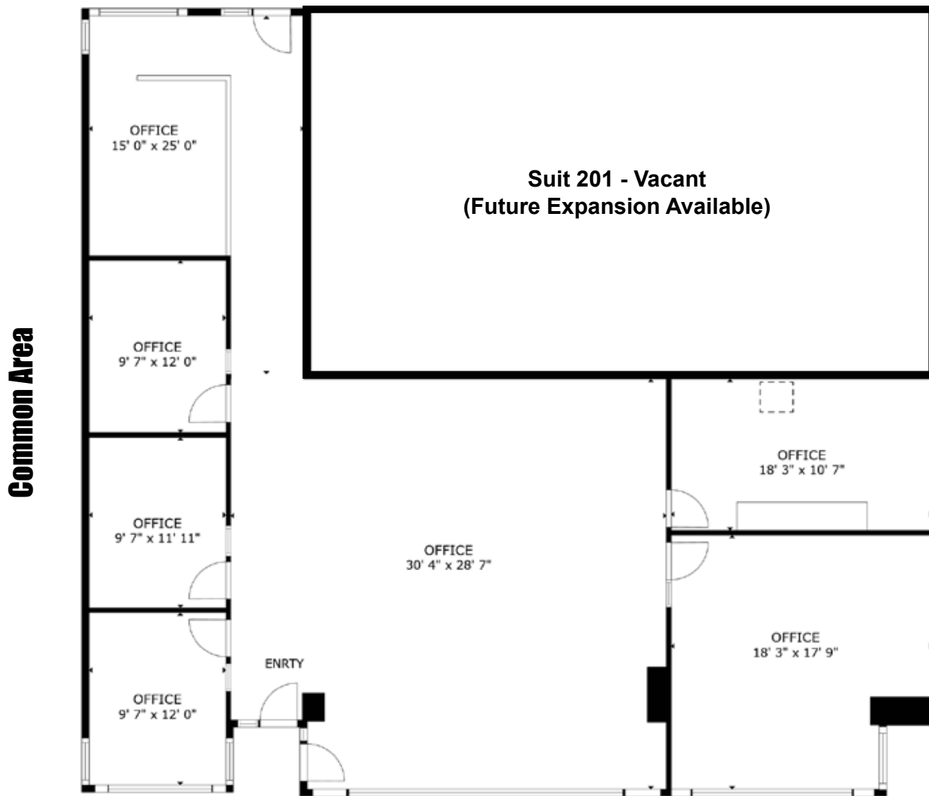
FLOOR PLAN
