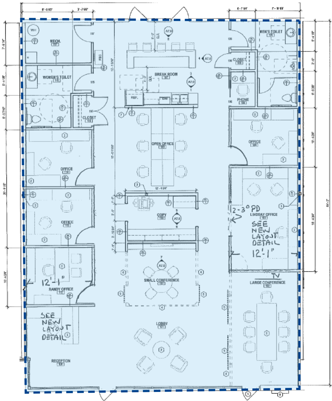
① NEW WORK FLOOR PLAN 1/4" = 1'-0"
