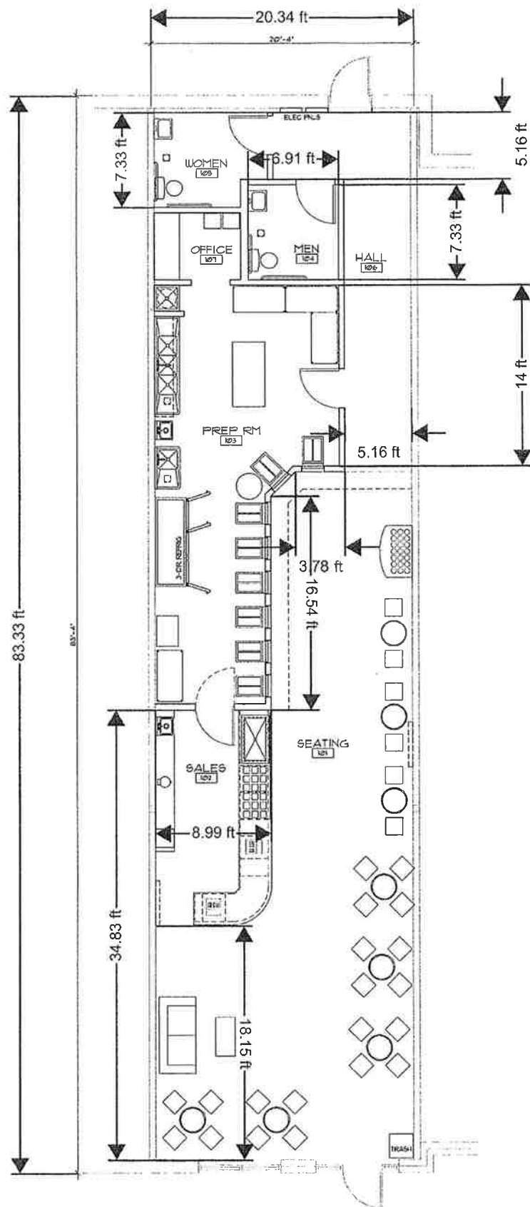
PLAN - SCHEME I Middleton, WI 02-24-12
