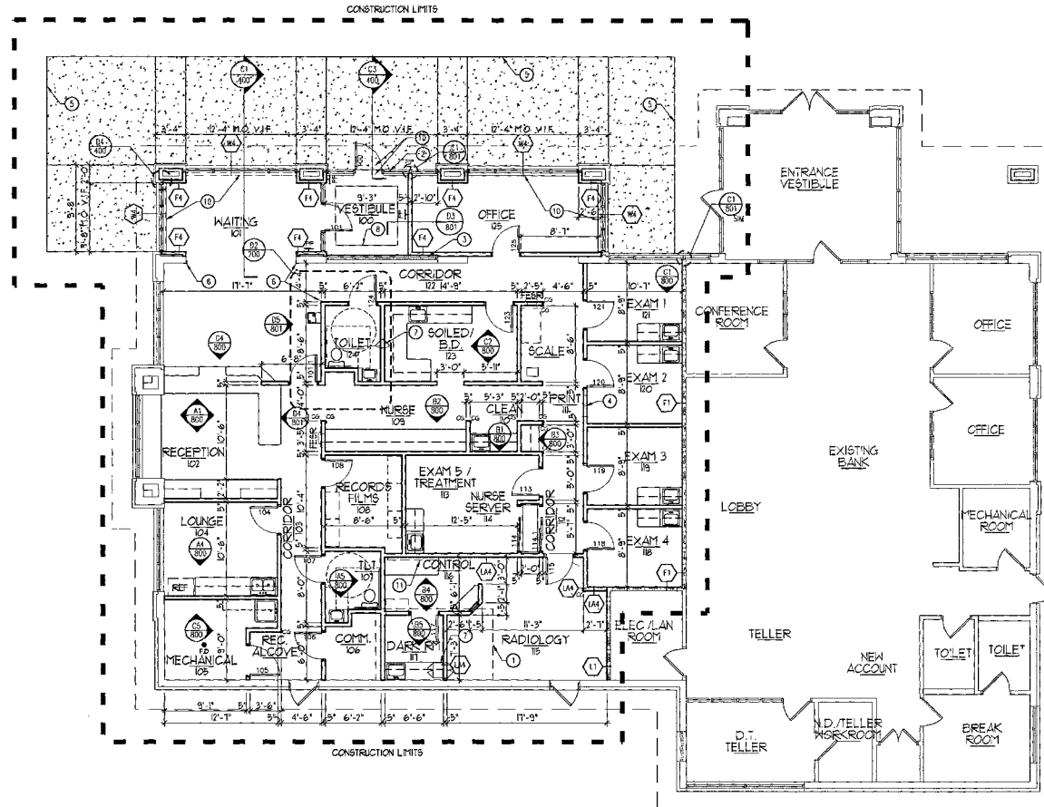
N FLOOR PLAN FIRST FLOOR ELEVATION: 926.50 1/8"=1'-0"
