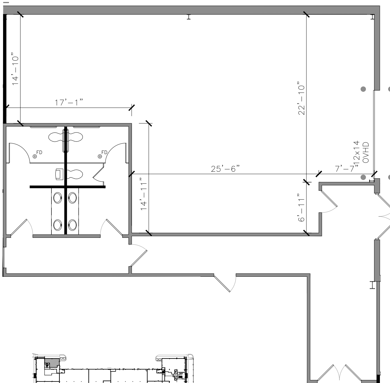
LOCATION PLAN
