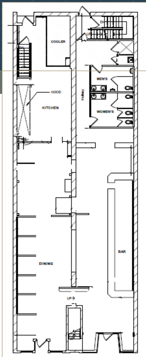
1 st Floor
