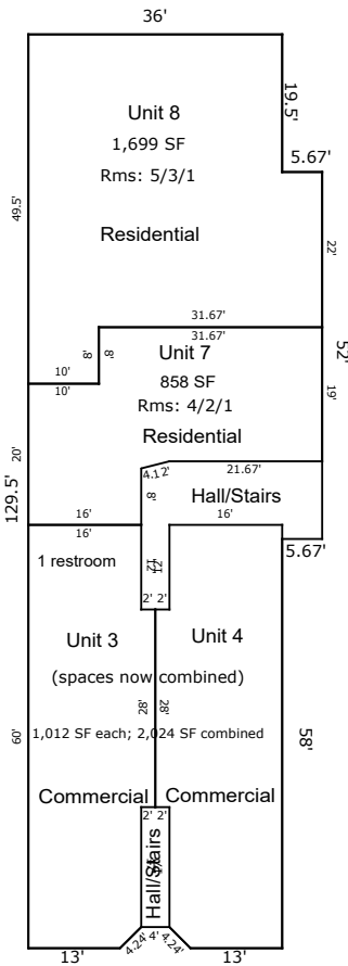
1st Floor
