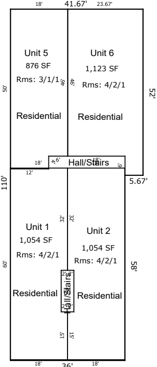
2nd Floor
