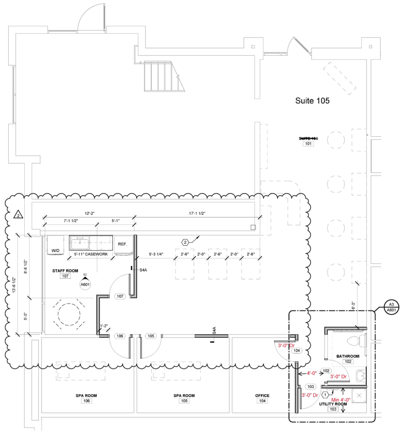
A2 FLOOR PLAN 1/4" = 1'-0"
