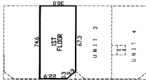
UNIT 2 1ST FLOOR AREA = 2,212 SQ. FT.
