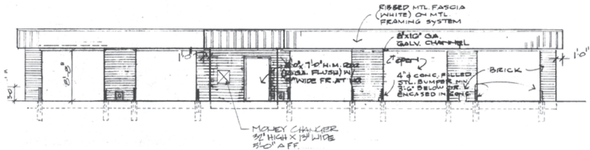
FRONT ELEVATION
