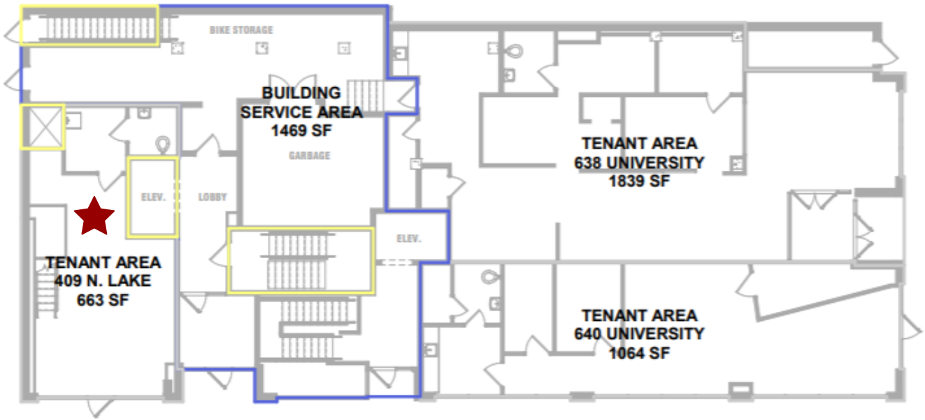
1 1ST FLOOR 1/8" = 1'-0"
