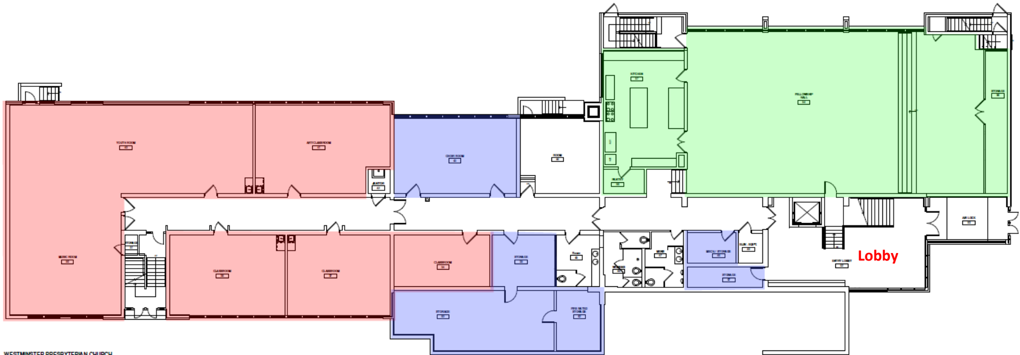
WESTMINSTER PRESBYTERIAN CHURCH Proposed Ground Floor Plan
