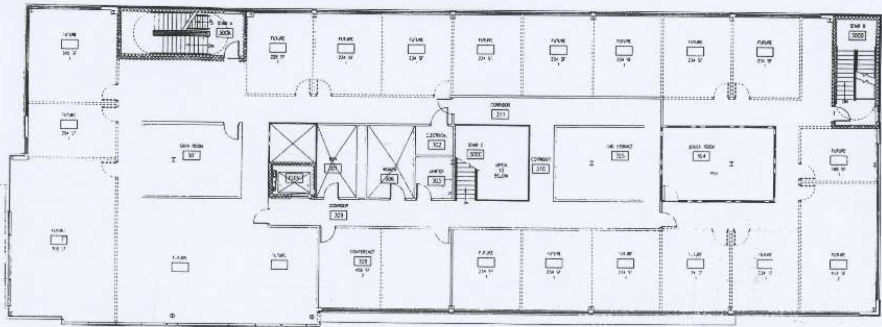
2 LEVEL 3 HVAC FLOOR PLAN 102 SCALE: 1/8" = 1'-0"
