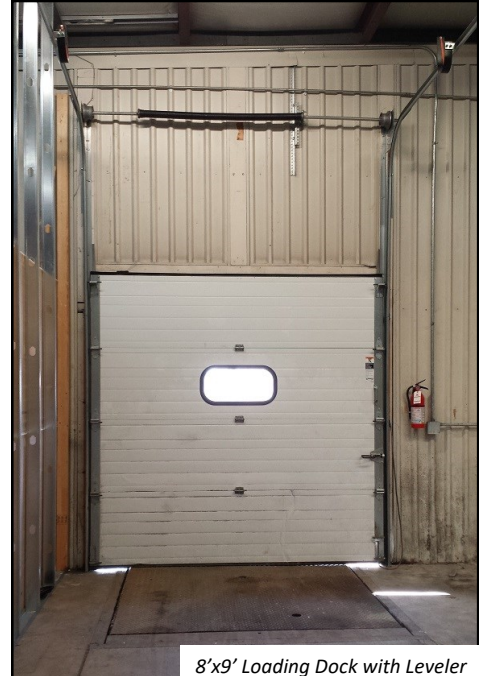
8'x9' Loading Dock with Leveler
