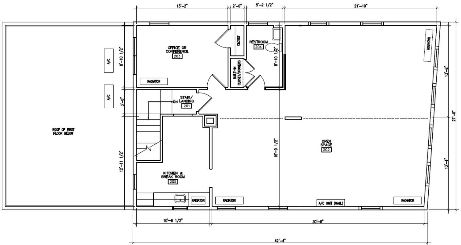
2 SECOND FLOOR PLAN - EXISTING 1/4"=1'-0"
