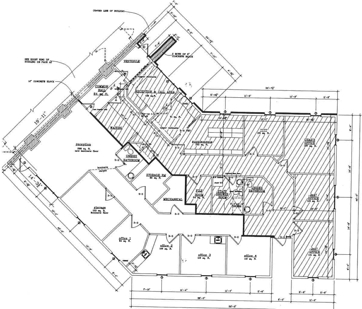
OFFICE FLOOR PLAN - LEFT WING 1/4" = 1'-0"
