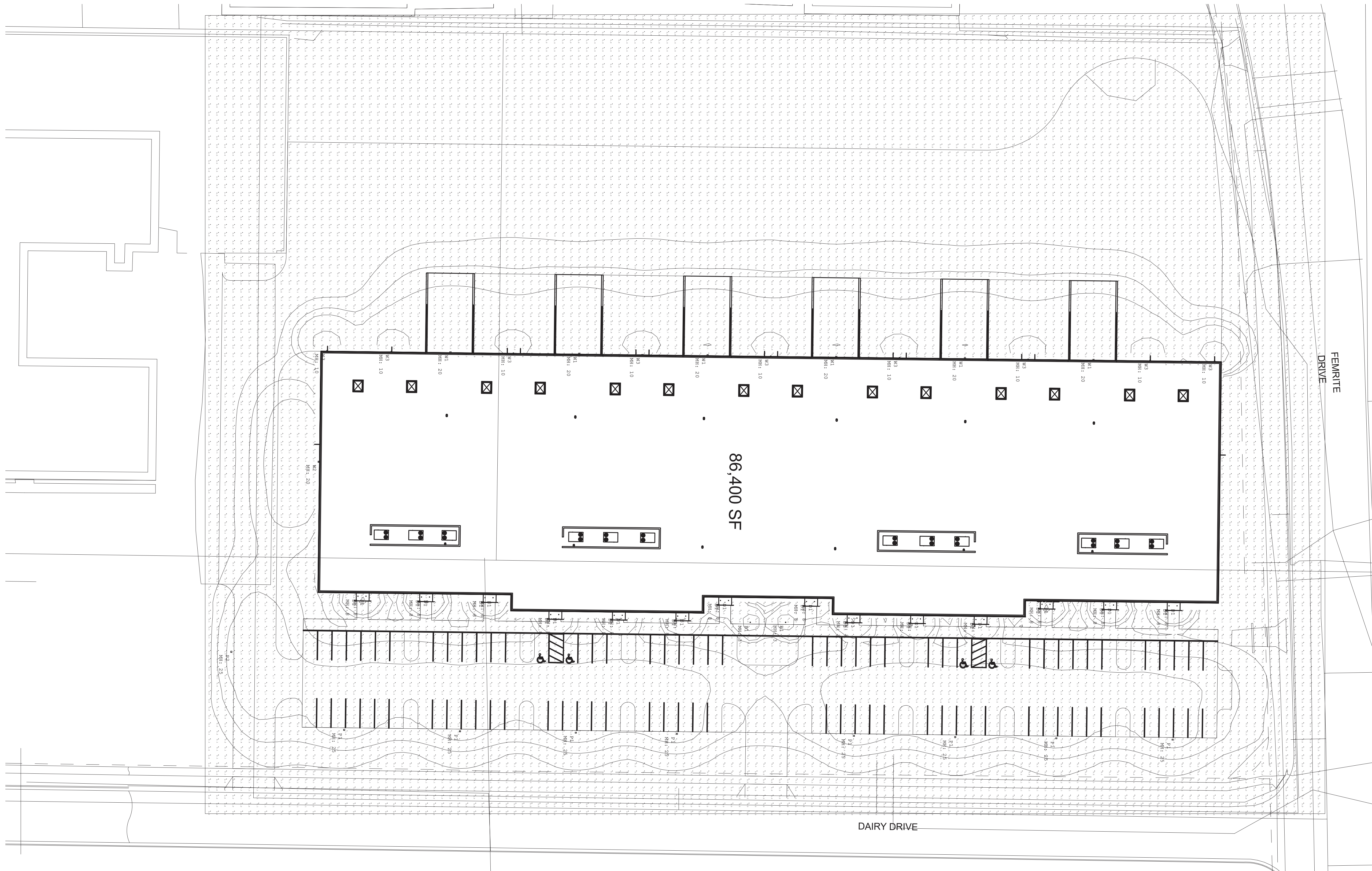
A1 SITE LIGHTING PLAN NOT TO SCALE
