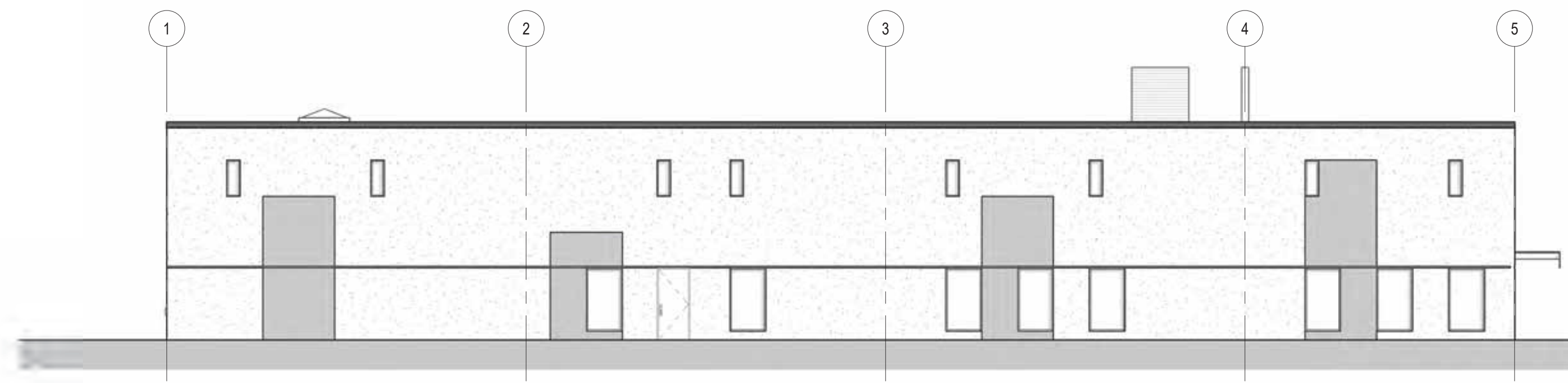
C1 SOUTH ELEVATION 3/32" = 1'-0"
