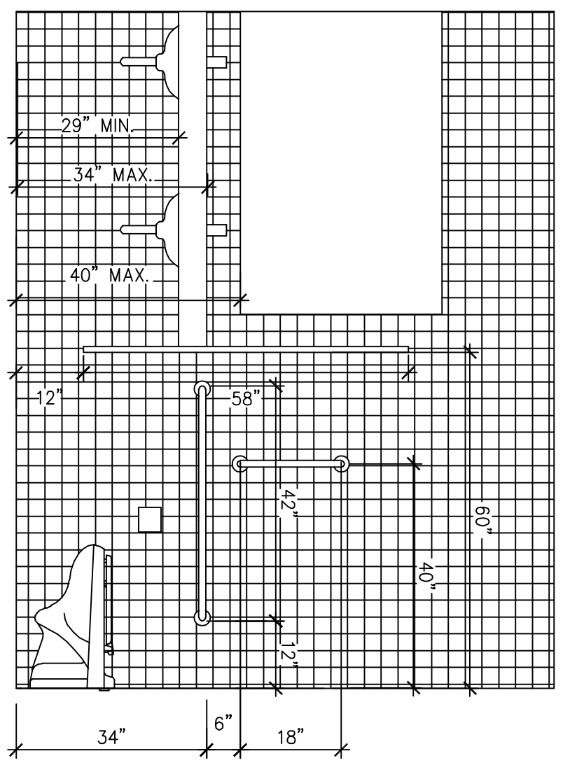
ELEVATION 1/2" = 1'-0"
